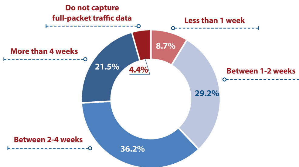
Figure 22: Retention practices for full-packet traffic data.
